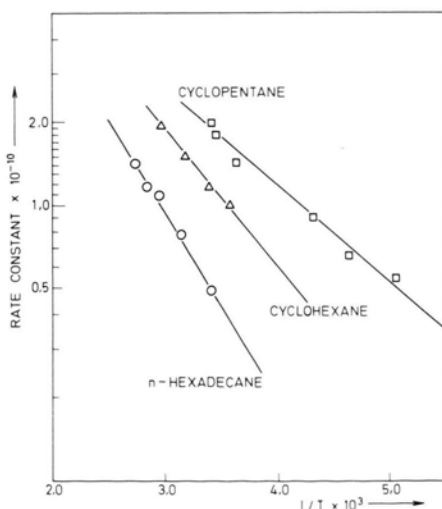
Fig. 1. Plots for activation energy determination of \text{R}^\bullet + \text{I}_2 reactions got by electron pulse radiolysis.
